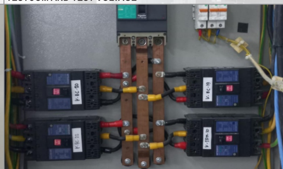
INCOMING PANEL 3P 220V
